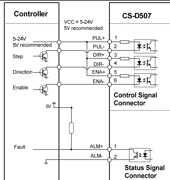
Figure 3: Connections to open-collector signal (common-anode)
